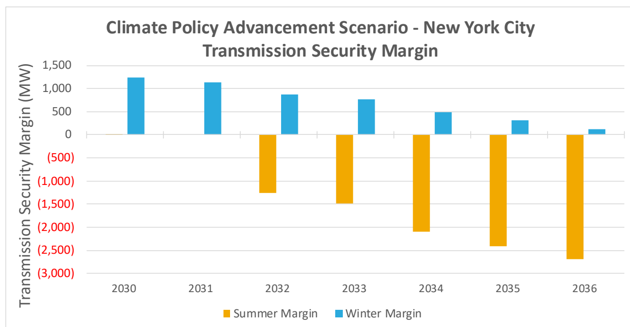
Figure 50: Climate Policy Advancement - New York City Transmission Security Margin
