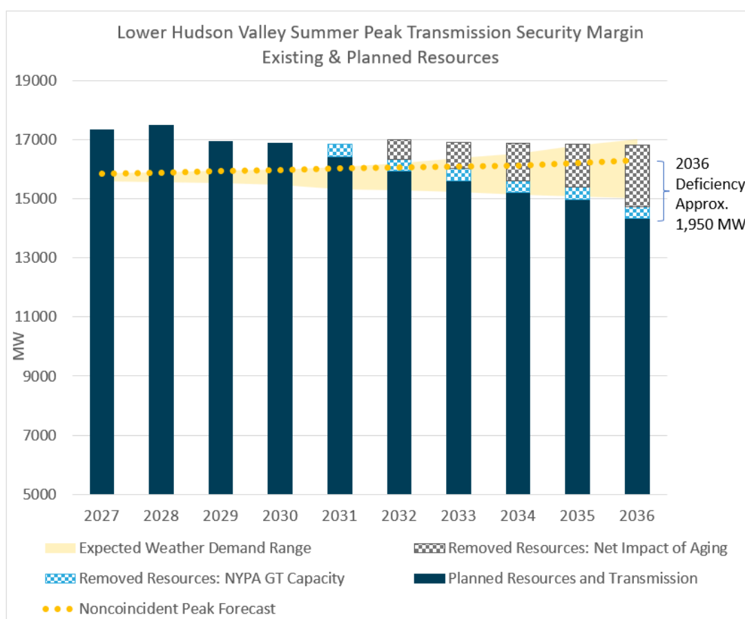
Figure 39: Lower Hudson Valley Summer Transmission Security Margin
