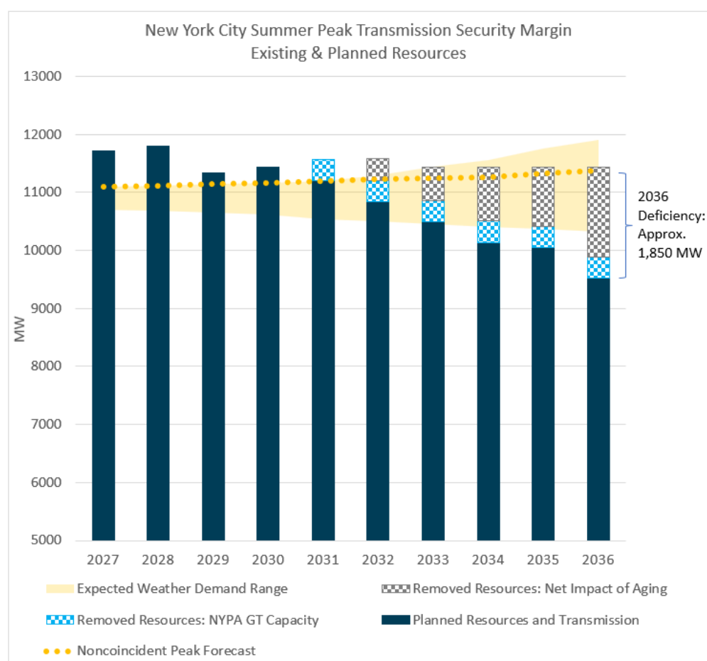
Figure 40: NYC Summer Peak Transmission Security Margin
