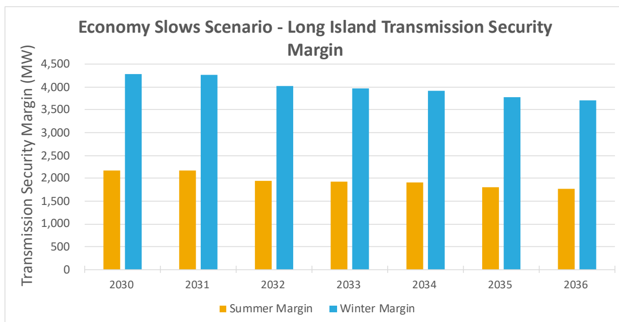
Figure 59: Economy Slows Scenario - Long Island Transmission Security Margin
