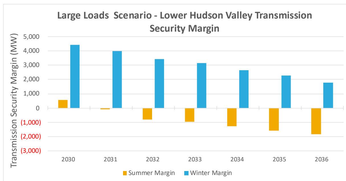
Figure 53: Large Loads Scenario - Lower Hudson Valley Transmission Security Margin
