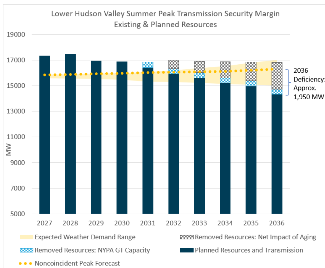
Figure 66: Lower Hudson Valley Summer Peak Transmission Security Margin
