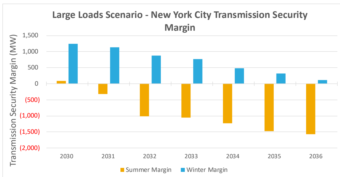
Figure 54: Large Loads Scenario - New York City Transmission Security Margin
