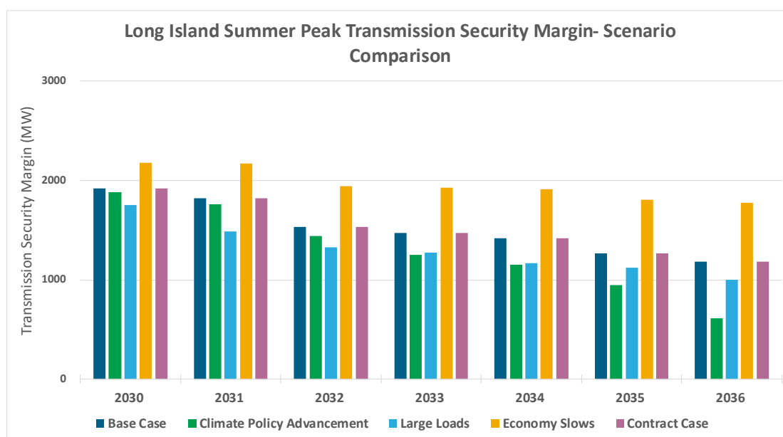
Figure 71: Scenario Summer Long Island Transmission Security Margins
