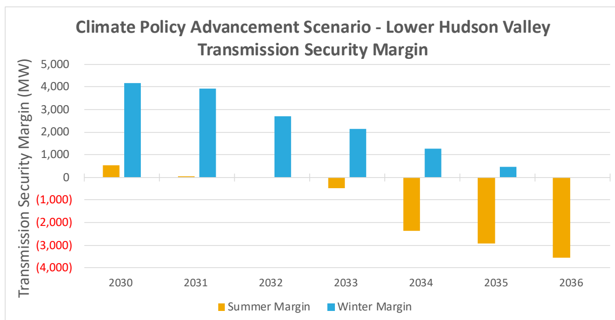
Figure 49: Climate Policy Advancement - Lower Hudson Valley Transmission Security Margin
