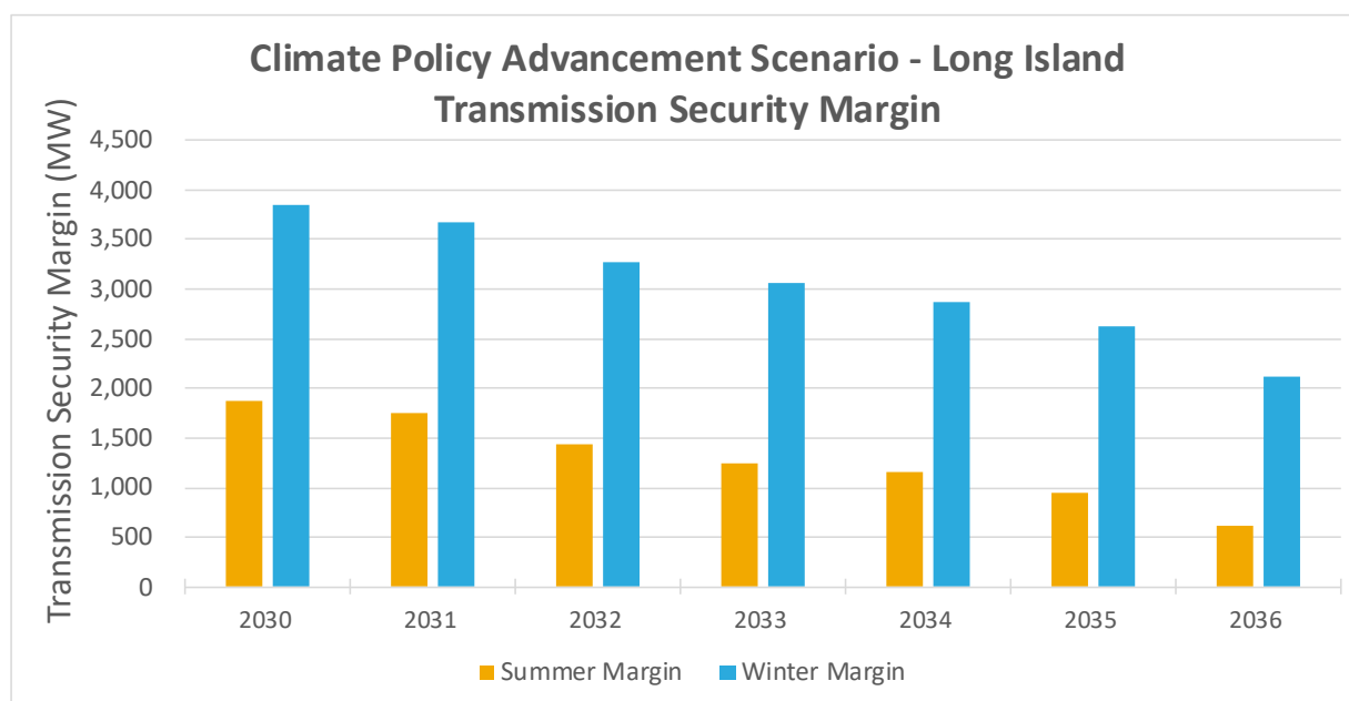
Figure 51: Climate Policy Advancement - Long Island Transmission Security Margin
