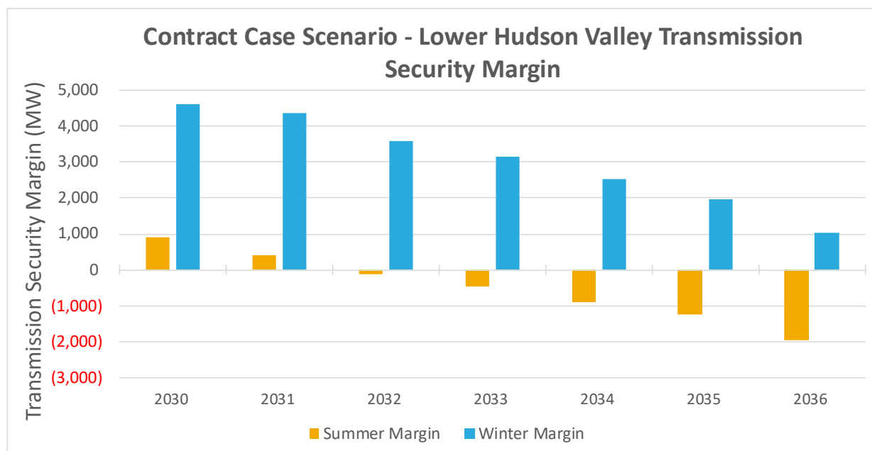
Figure 61: Contract Case Scenario - Lower Hudson Valley Transmission Security Margin
