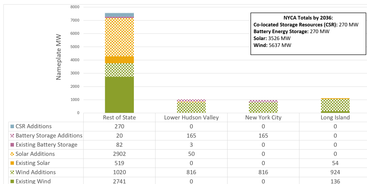
Figure 24: Planned 2036 Zero-Emission Fuel Mix by Zone
