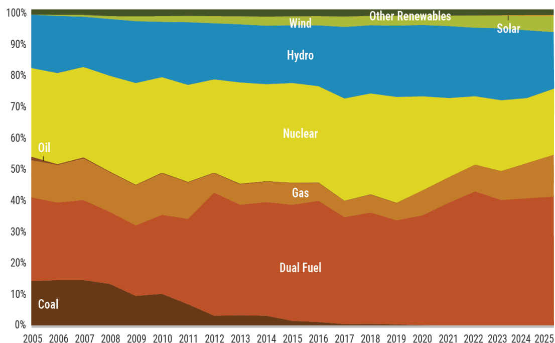
Figure 7: Historical Generating Capacity Fuel Mix in New York State
