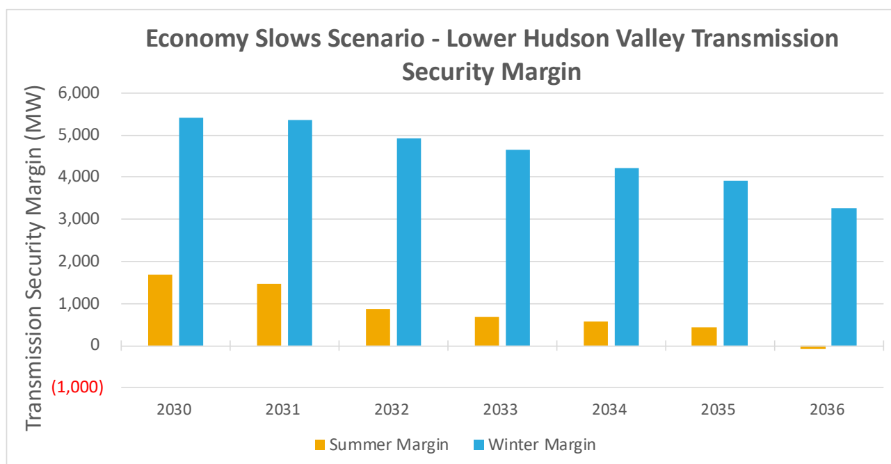
Figure 57: Economy Slows Scenario - Lower Hudson Valley Transmission Security Margin
