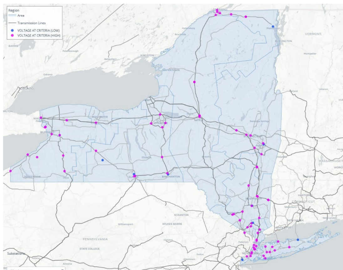
Figure 43: State Electric Map Highlighting Voltage Issues
