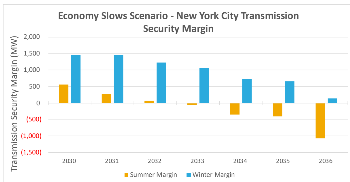
Figure 58: Economy Slows Scenario - New York City Transmission Security Margin
