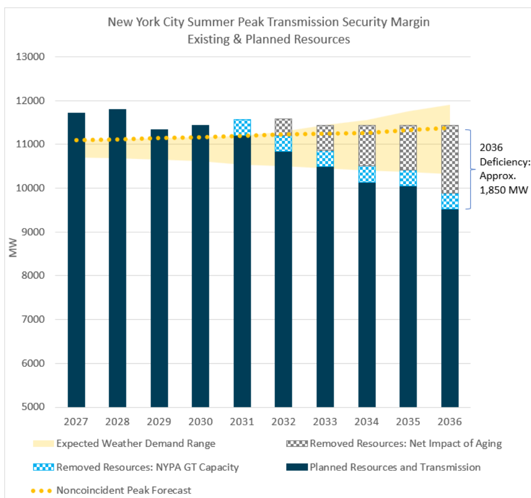
Figure 67: NYC Summer Peak Transmission Security Margin
