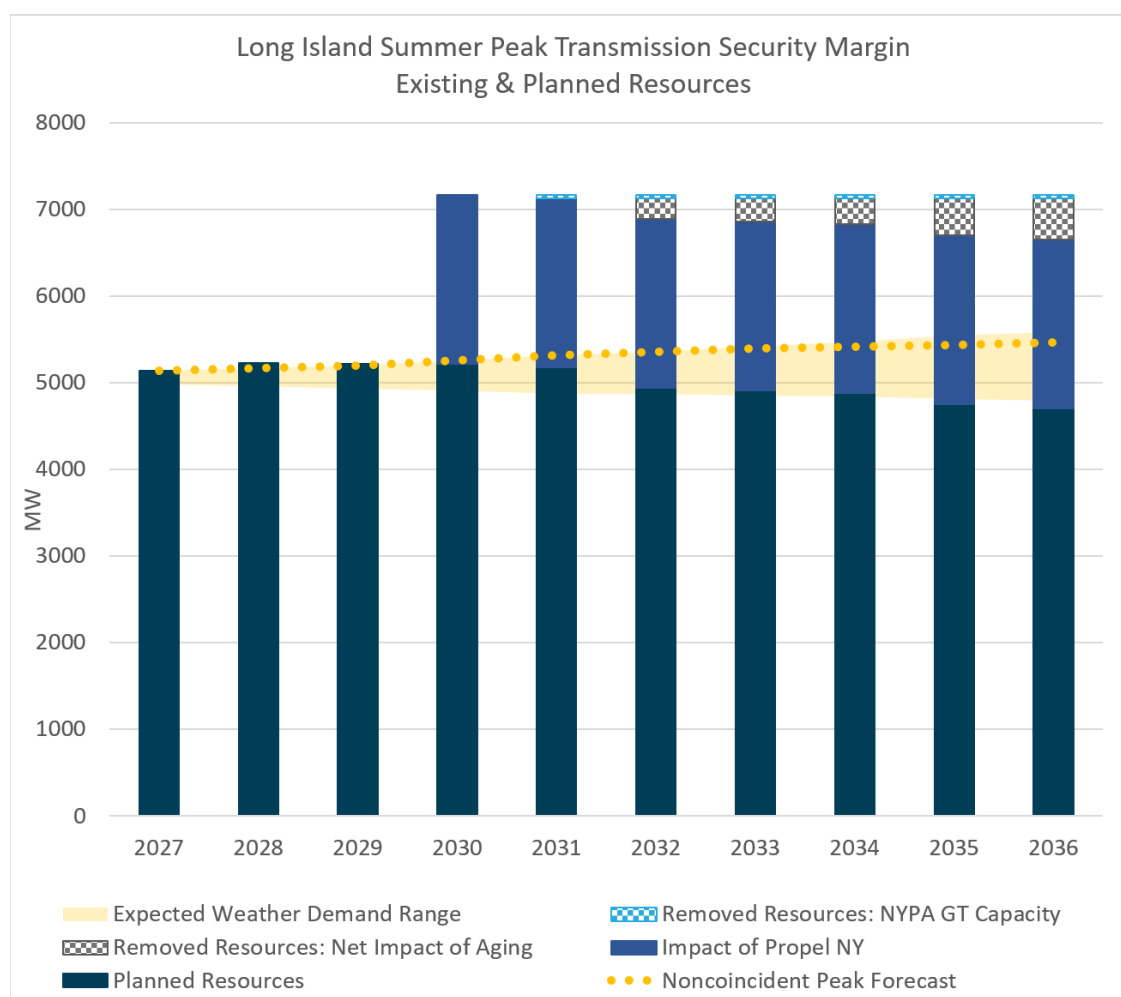
Figure 41: Long Island Summer Peak Transmission Security Margin
