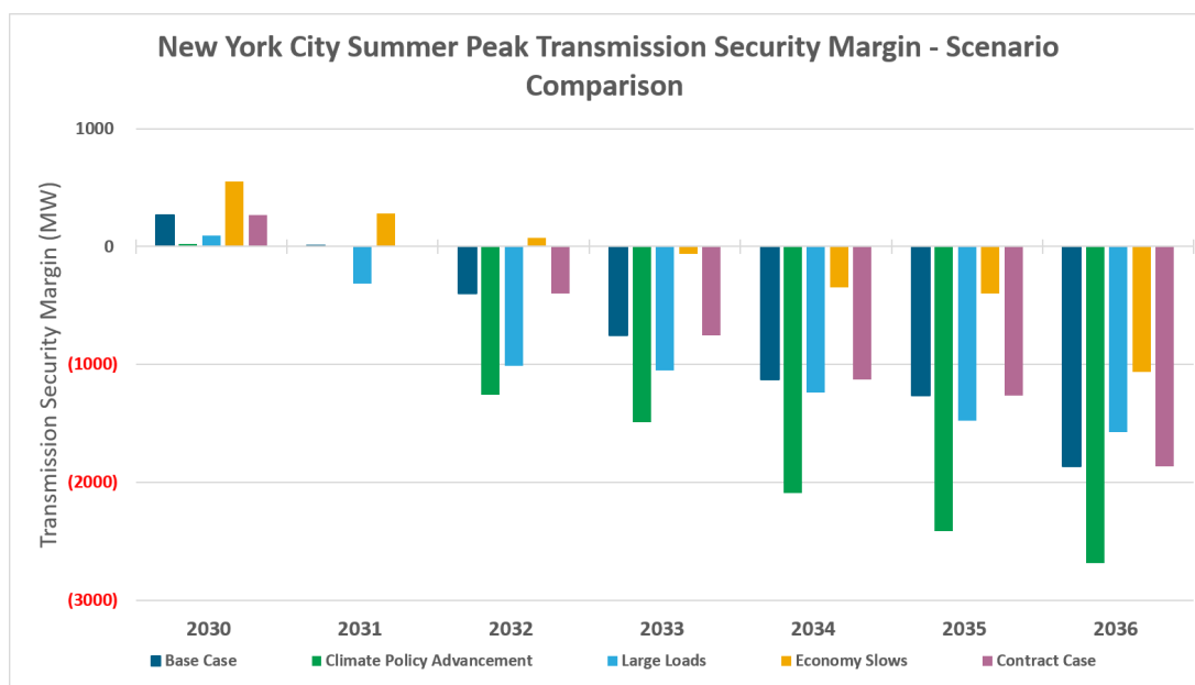
Figure 70: Scenario Summer New York City Transmission Security Margin
