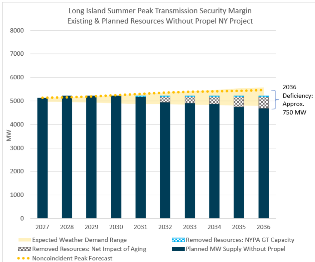
Figure 42: Long Island Transmission Security Margin without Propel NY
