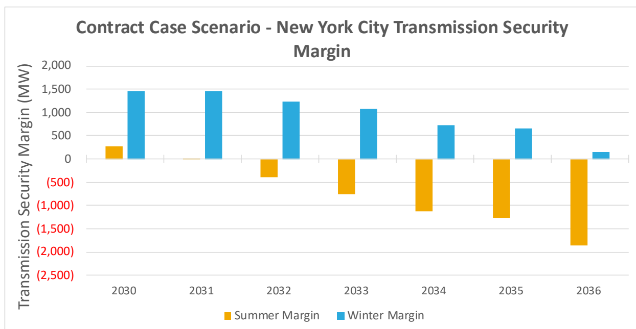
Figure 62: Contract Case Scenario - New York City Transmission Security Margin
