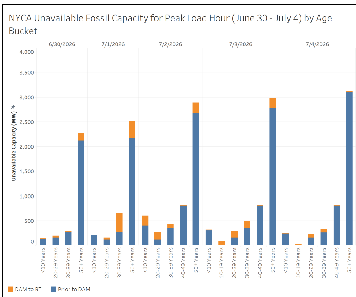
Figure 9: Unavailable Capacity by Unit Age in the July Heatwave
