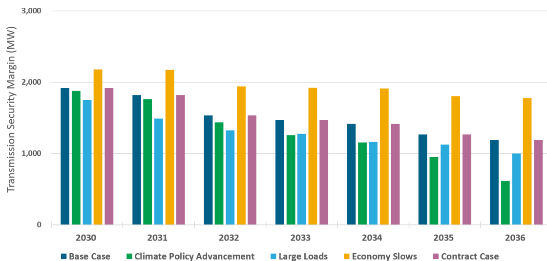
Figure 72: Scenario Summer Long Island Transmission Security Margins
