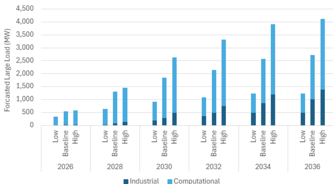
Figure 21: RNA Large Load Forecast Summer Coincident Peak by Load Type (MW)
