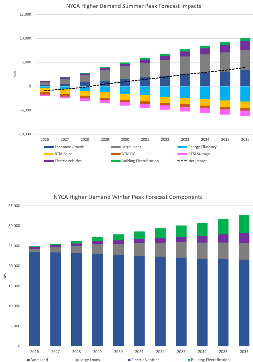
Figure 17: NYCA Higher Demand Summer and Winter Peak Forecast Impacts
