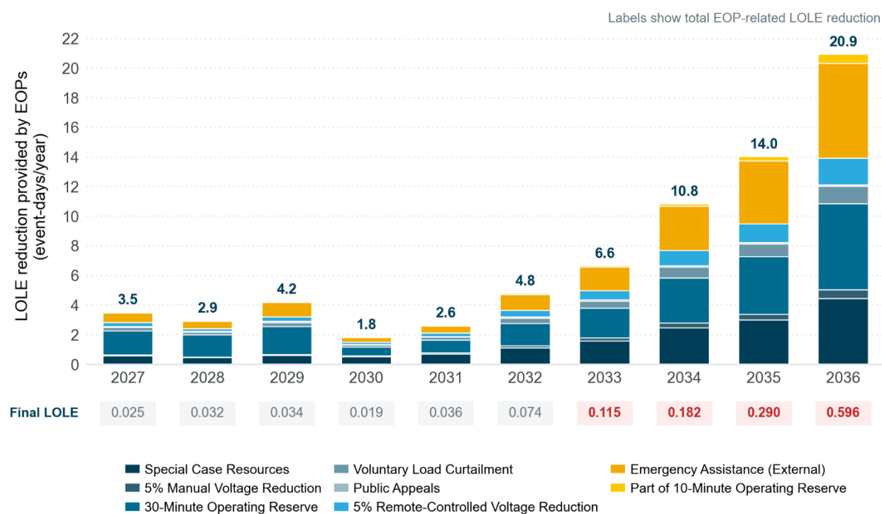
Figure 36: Resource Adequacy Contribution by Emergency Operating Procedure
