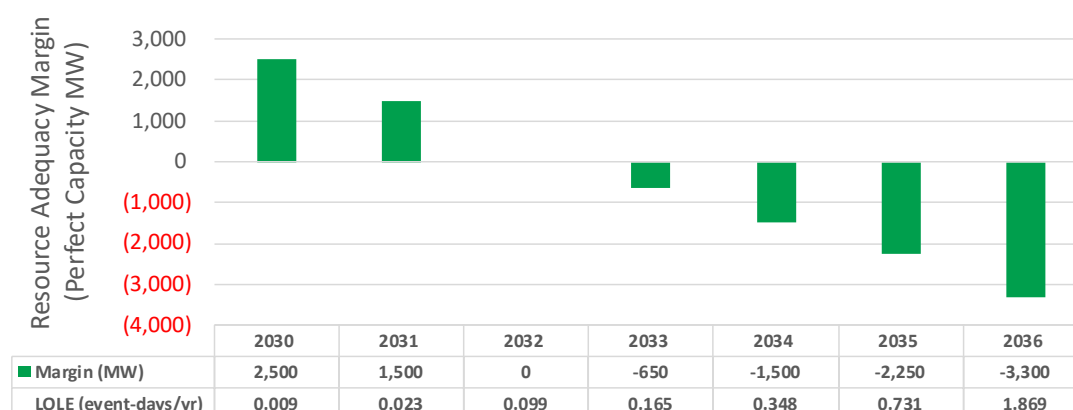
Figure 48: Climate Policy Advancement - Resource Adequacy
