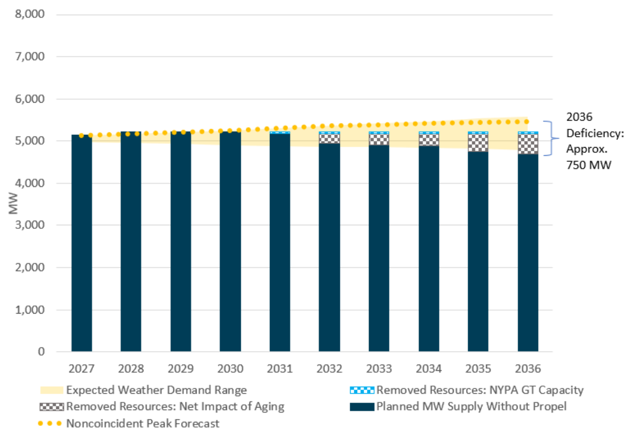
Figure 42: Long Island Transmission Security Margin without Propel NY
