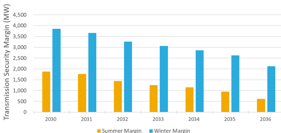
Figure 51: Climate Policy Advancement - Long Island Transmission Security Margin
