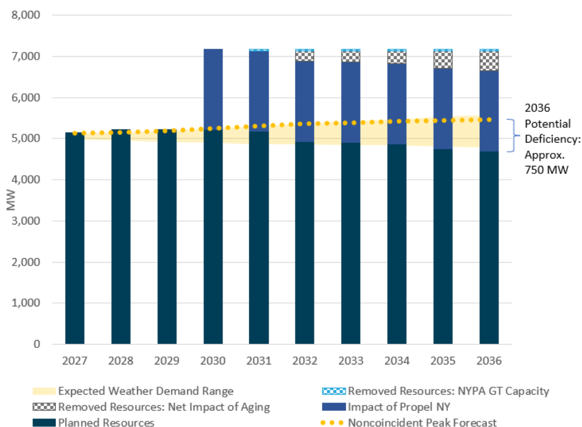
Figure 41: Long Island Summer Peak Transmission Security Margin – Existing & Planned Resources
