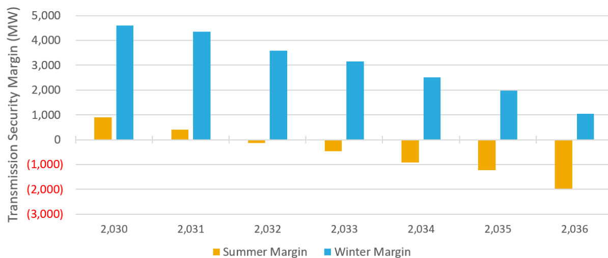
Figure 62: Contract Case Scenario - New York City Transmission Security Margin
