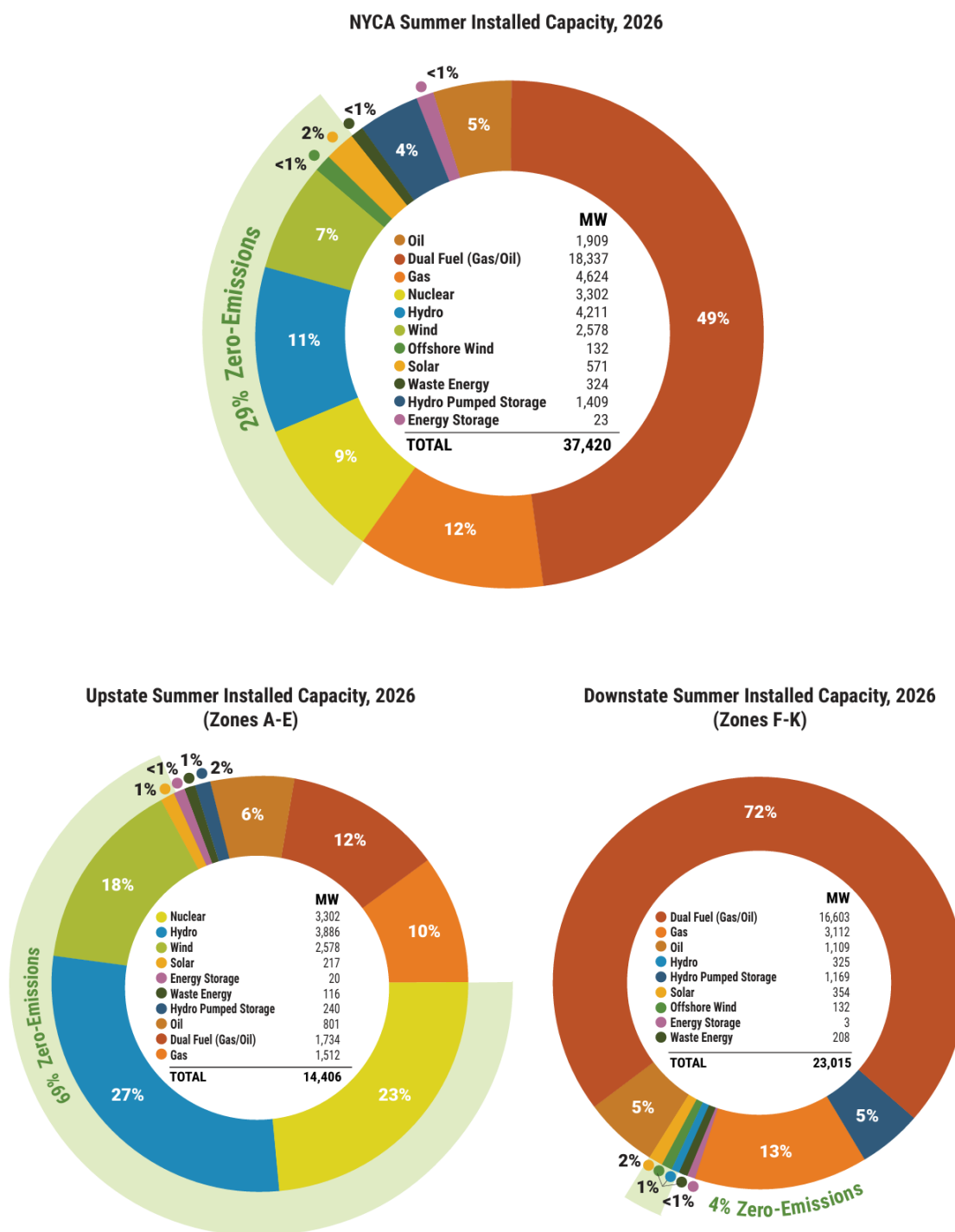
Figure 4: Summer Installed Capacity by Fuel Source — Statewide, Upstate, and Downstate New York: 2026
