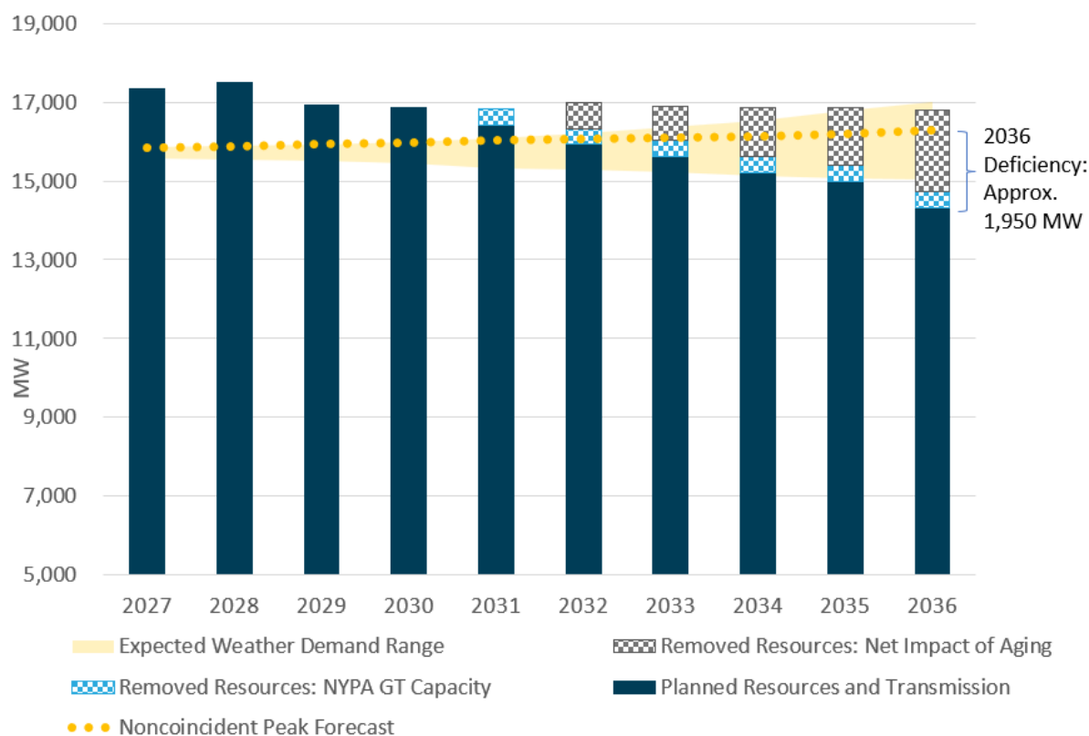
Figure 67: Lower Hudson Valley Summer Peak Transmission Security Margin – Existing & Planned Resources
