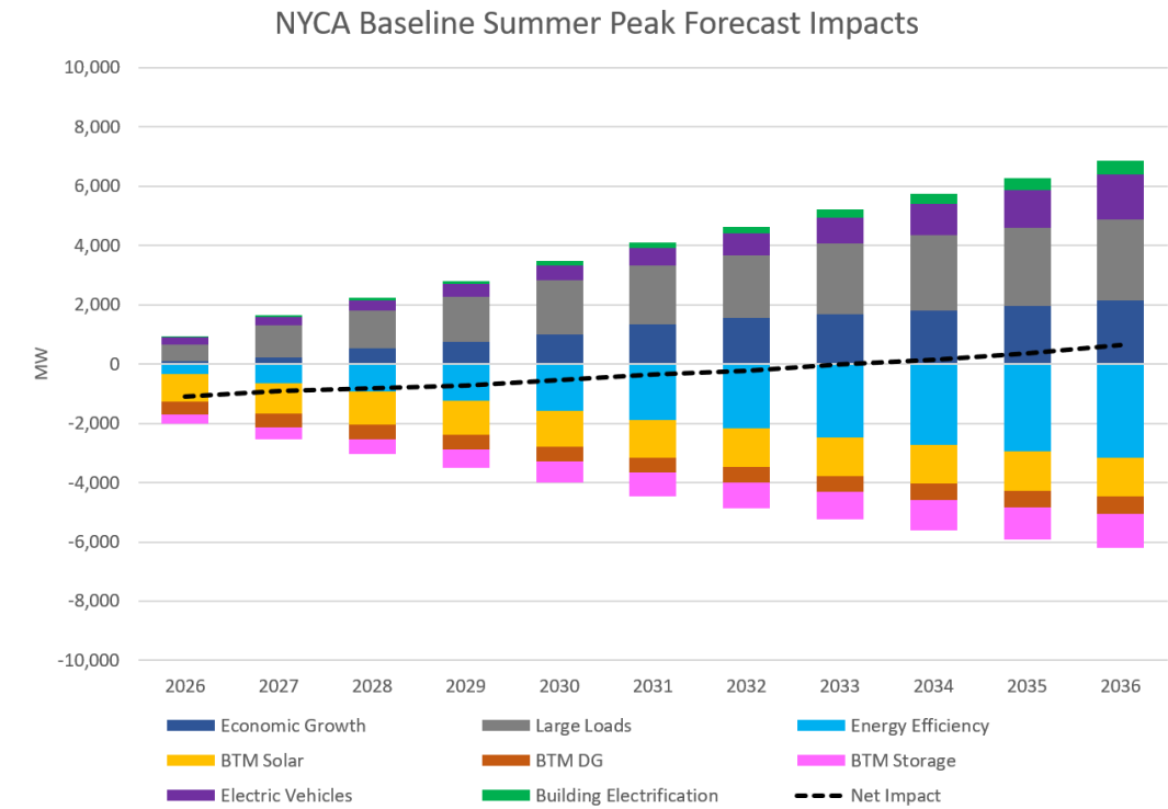
Figure 16: NYCA Baseline Summer and Winter Peak Forecast Impacts
