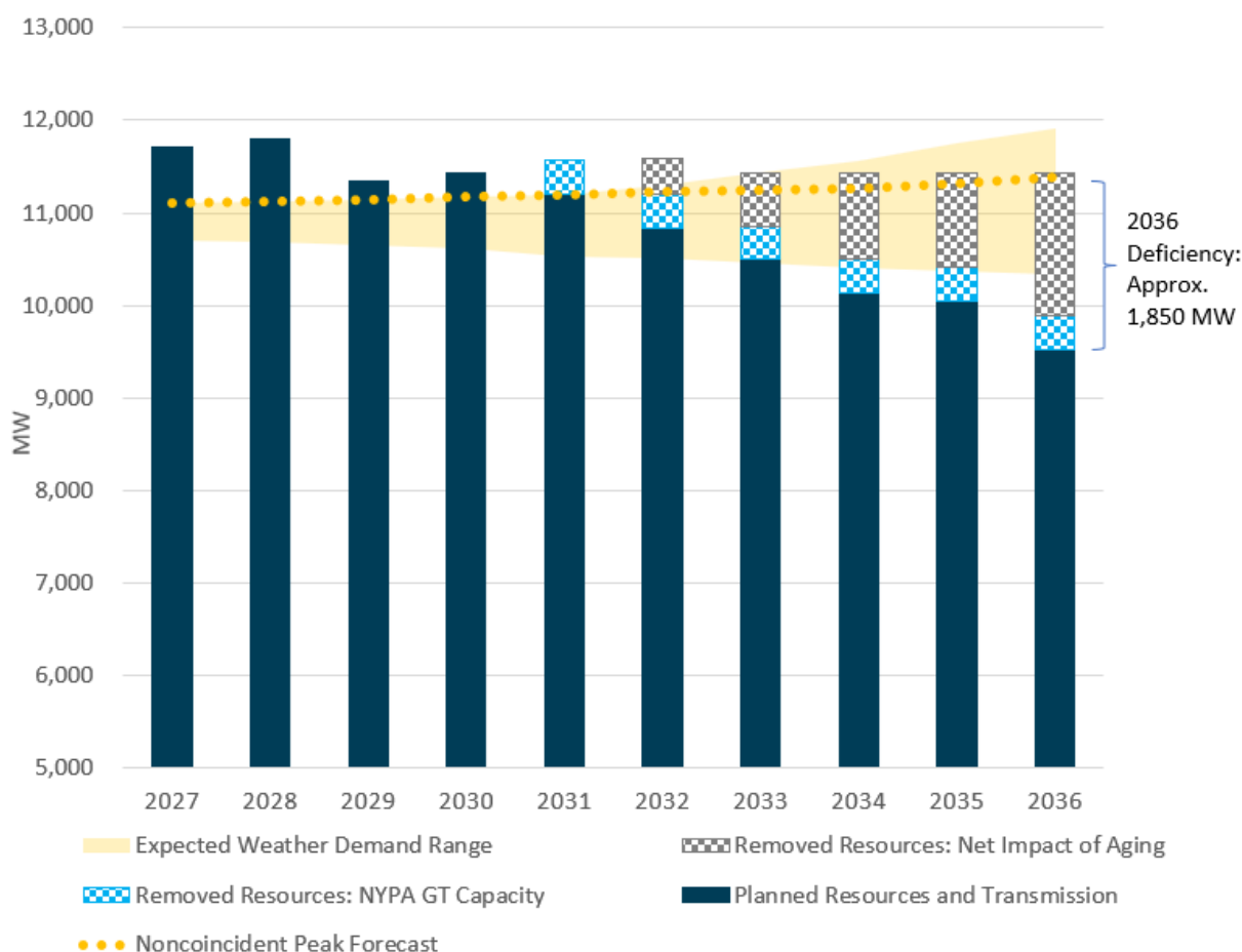
Figure 68: NYC Summer Peak Transmission Security Margin – Existing & Planned Resources
