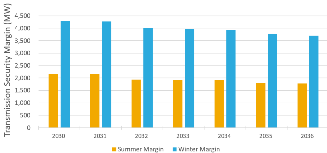
Figure 59: Economy Slows Scenario - Long Island Transmission Security Margin
