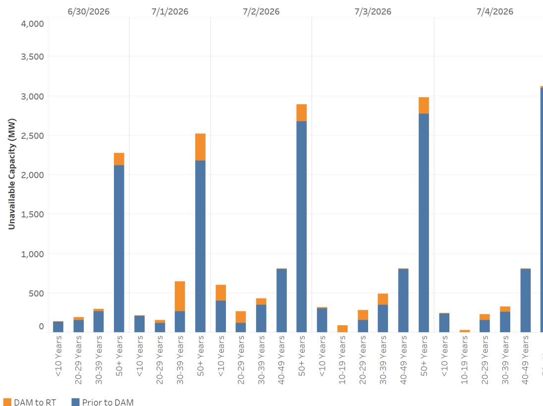
Figure 9: Unavailable Capacity by Unit Age in the July Heatwave
