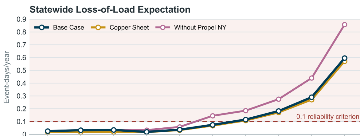
Figure 38: Resource Adequacy Impact of the Propel NY Project
