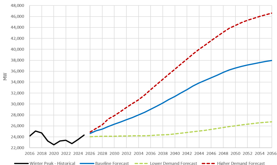
Figure 15: 30-Year NYCA Winter Peak Forecast – Coincident Peak
