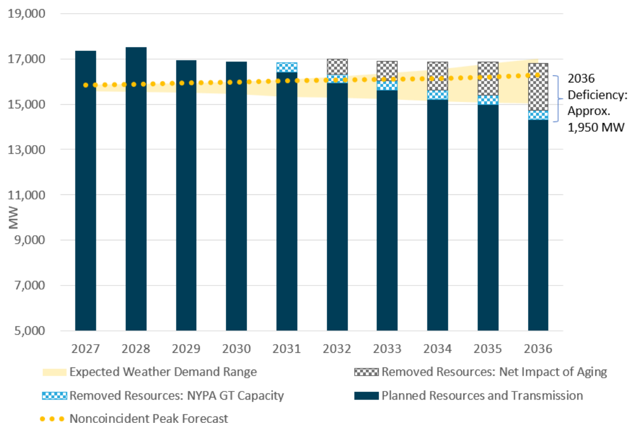
Figure 39: Lower Hudson Valley Summer Transmission Security Margin – Existing & Planned Resources
