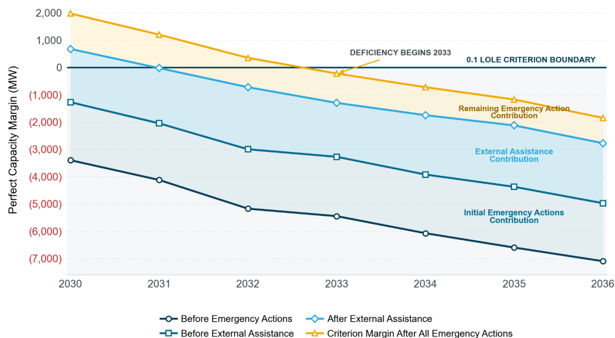
Figure 37: Statewide Resource Adequacy Margin by Emergency Operating Procedure
