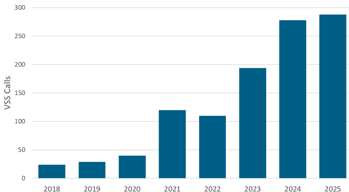
Figure 8: Voltage Support Service Calls in Recent Operations
