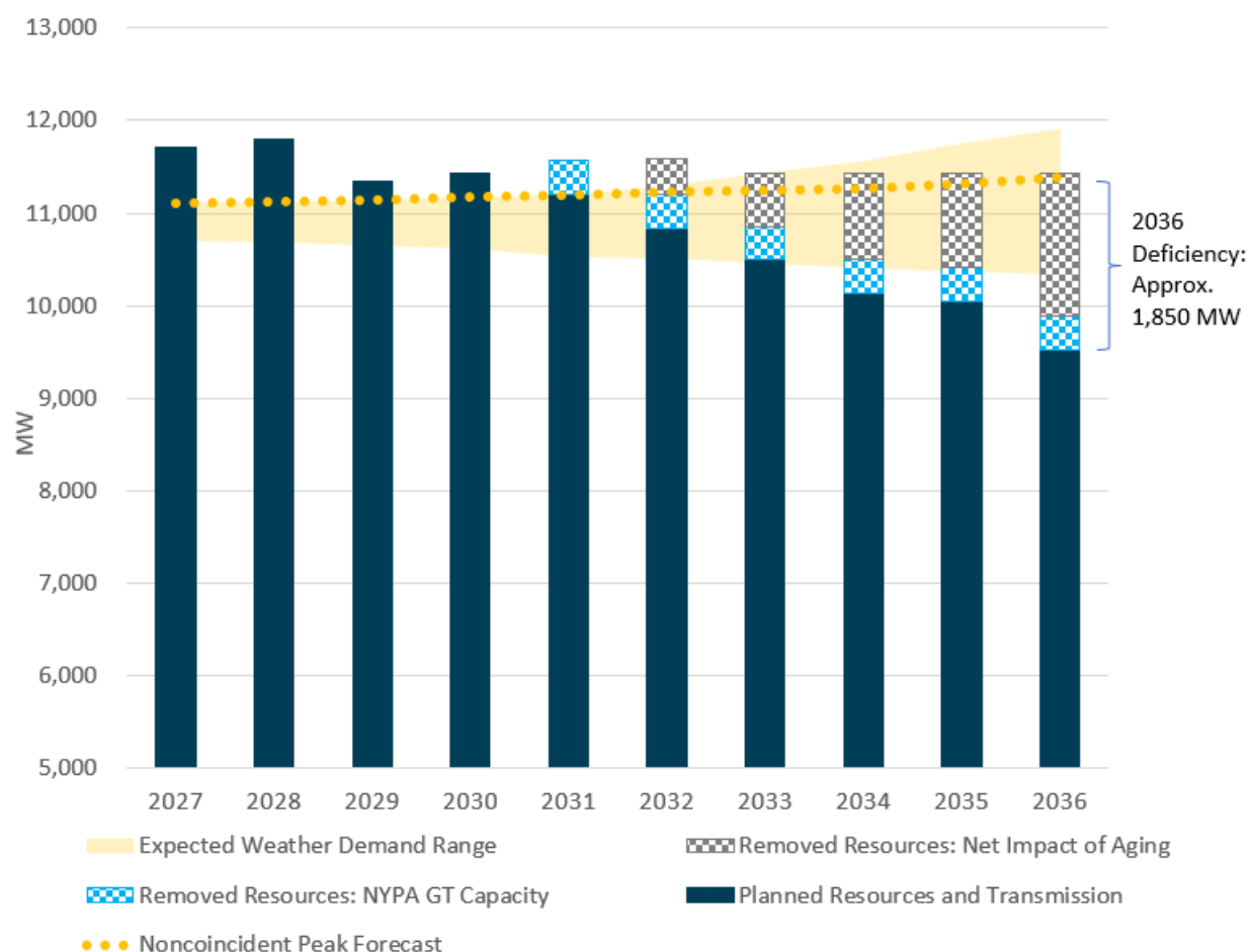
Figure 40: NYC Summer Peak Transmission Security Margin – Existing & Planned Resources
