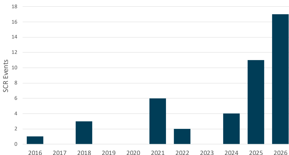
Figure 10: NYISO Activated SCR Calls (Excluding Tests) in Recent Operating History
