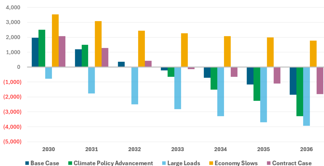
Figure 69: Scenario Resource Adequacy Margin
