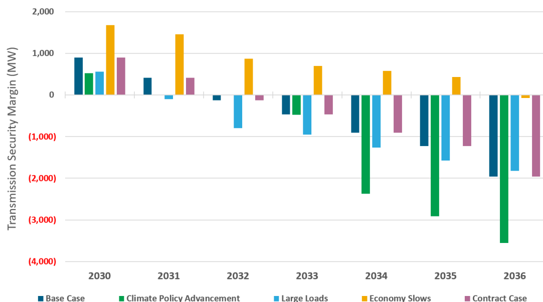
Figure 70: Scenario Summer Lower Hudson Valley Transmission Security Margin
