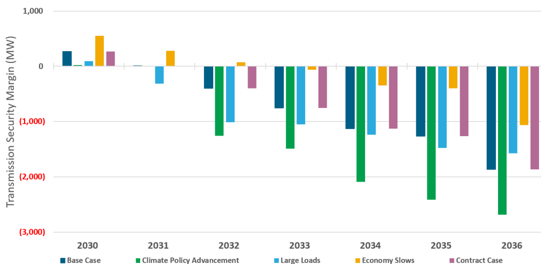
Figure 71: Scenario Summer New York City Transmission Security Margin
