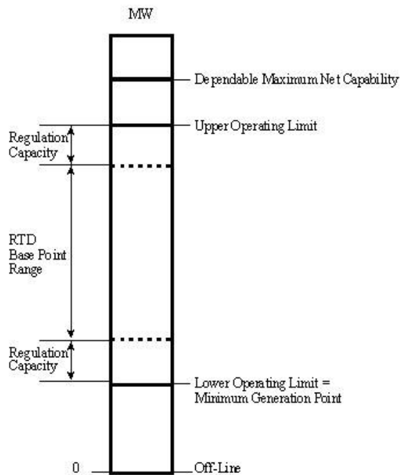
Figure 6: Generating Unit Operating Characteristics
